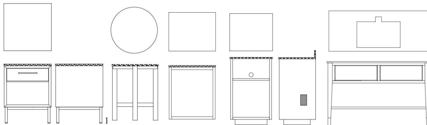
PC-206 Night Stand 20" x 20" x 25"
