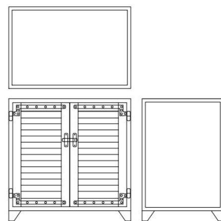
CO-104 Chest 36" x 23 7/8" x 36"
