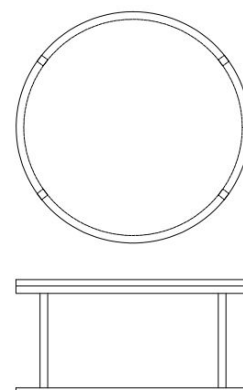
CO-107 Round Cocktail Table 36" dia x 18"
