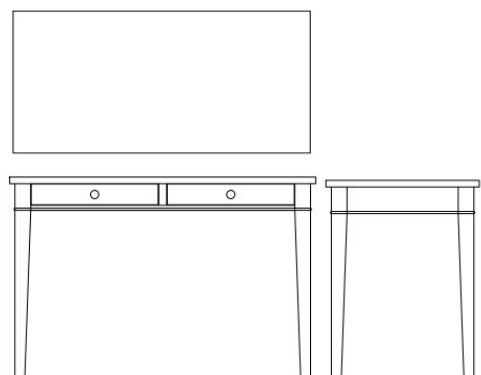
CO-105 Desk 68" x 23 1/4" x 37 5/8"
