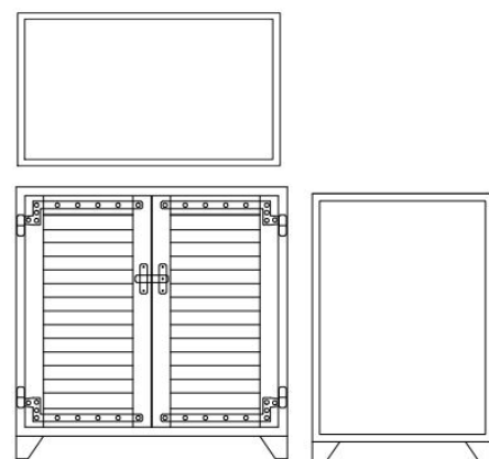
BG-202 Chest 36" x 23 7/8" x 36"
