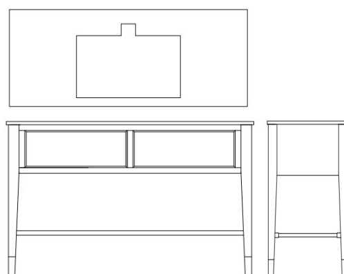
BG-800 Vanity 55" x 21 1/2" x 34 1/2"
