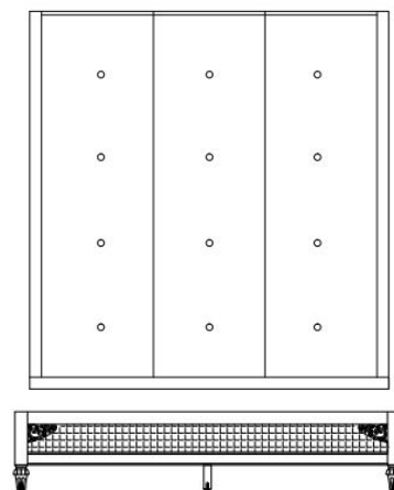
BG-100B King Platform 73 5/8" x 81 1/2" x 18 1/2" BG-101B Queen Platform 62" x 81 1/2" x 18 1/2"
