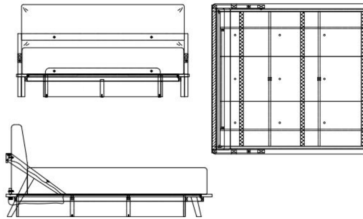
FZ-100 King Bed 76 7/8" x 93 1/4" x 41 1/2" FZ-101 Queen Bed 64 7/8" x 93 1/4" x 41 1/2"
