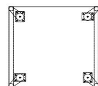
FZ-204 PTAC Cover 45 1/4" x 18 7/8" x 26 3/4"
