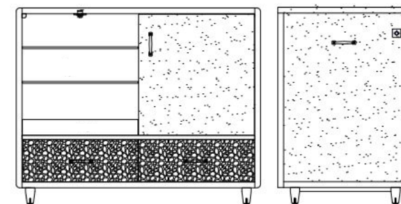
FZ-205 Hospitality Cabinet 46 1/2" x 25" x 37 1/4"
