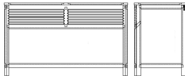
FZ-204 PTAC Cover 45 1/4" x 18 7/8" x 26 3/4"
