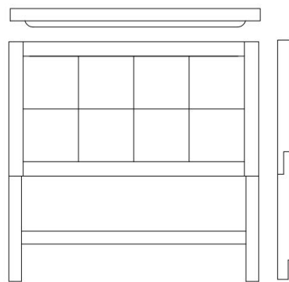
EV-104 King Headboard 74 1/2 x 3 x 58 1/2 EV-105 Queen Headboard 62" x 3" x 58 1/2"
