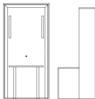
EV-107 Vertical Twin Murphy Bed w/ Desk 41 1/8" x 14 5/8" x 85 5/8"
