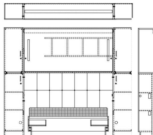
EV-102 King Stationary w/ Twin Murphy Bed 118" x 14 5/8" x 100"
